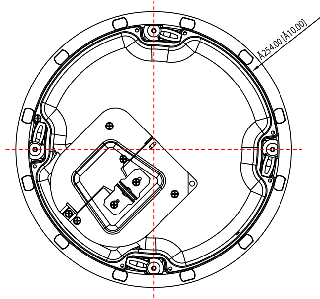
BACK/MINIMUM CUTOUT
